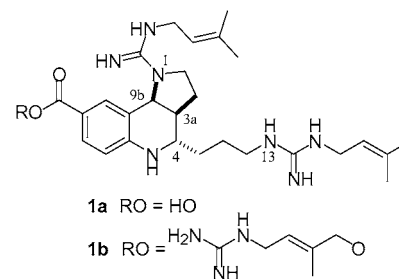
Figure 1. Martinella alkaloids (IUPAC numbering).
